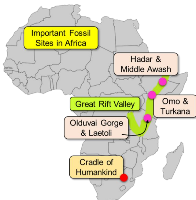
Figure 31: Location of the Rift Valley in East Africa.
