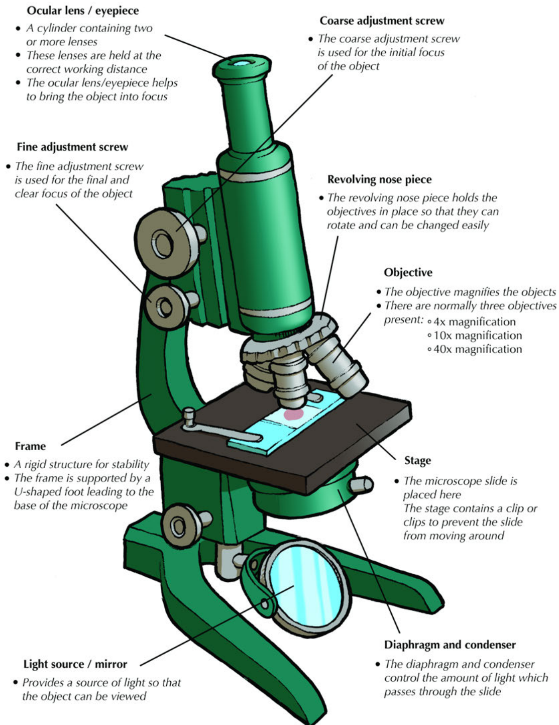
Figure 3.5: Light microscope
