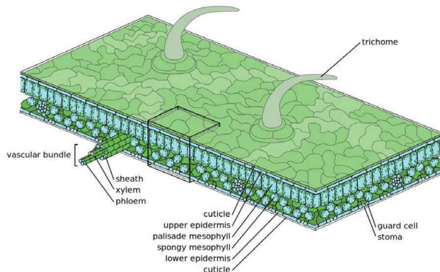
Figure 5.42: Leaf structure.
