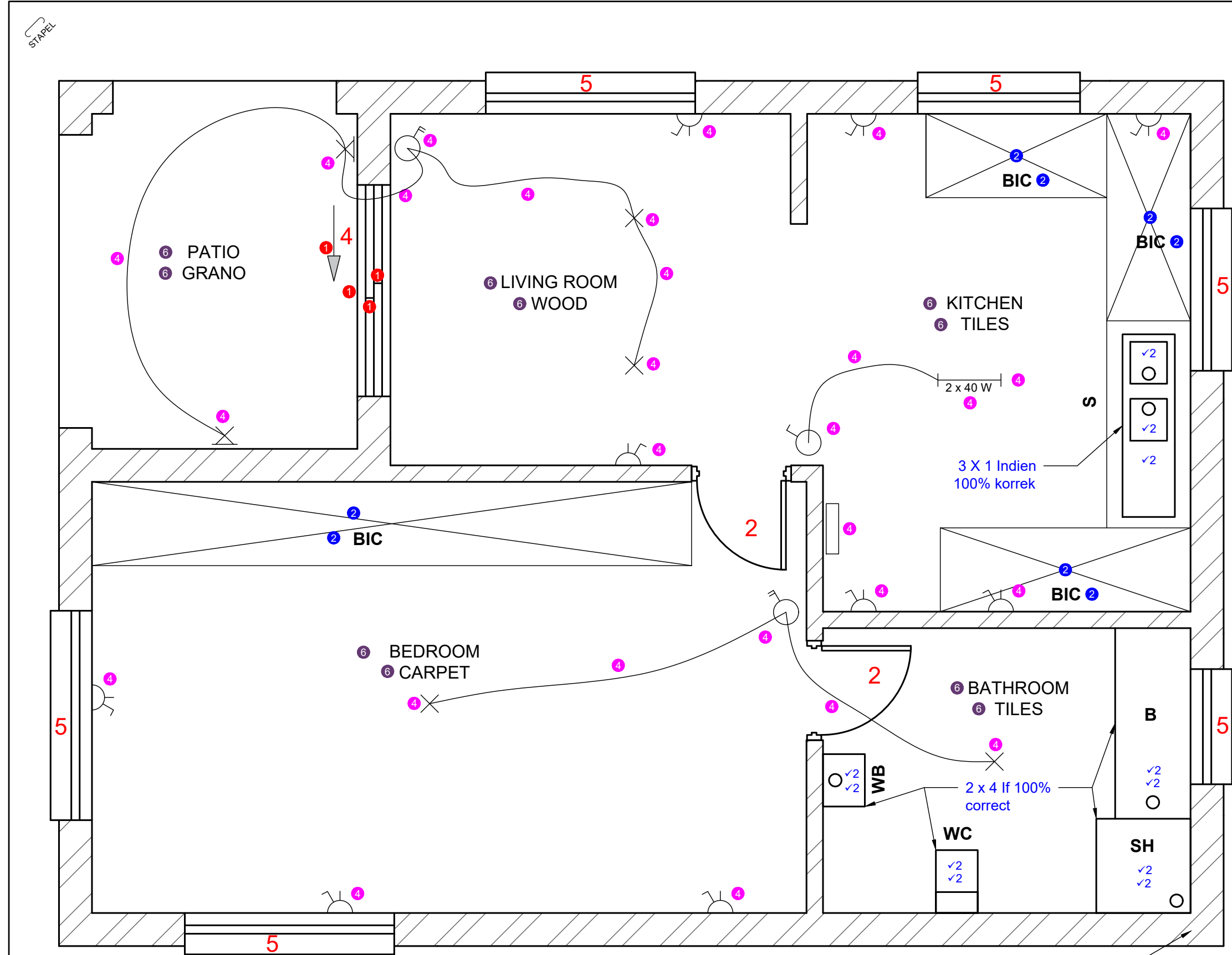
6 FLOOR PLAN 6 SCALE 1:40
