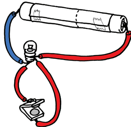
Figure 15.16 The bulb stops glowing when you press the switch. What is wrong?
