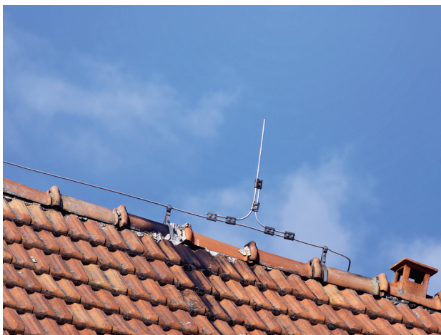
Lightning rod wire on a roof of clay tiles
