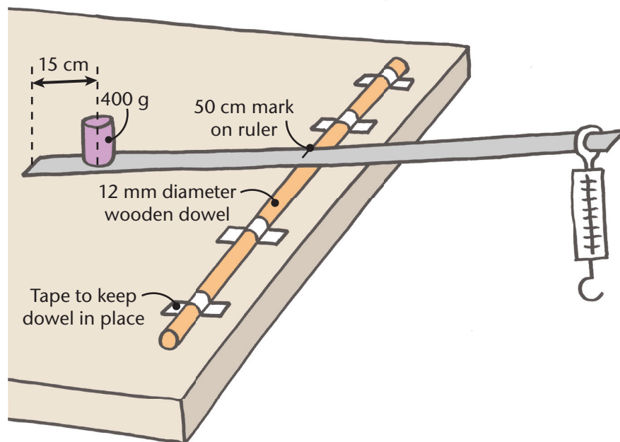
Figure 6.18 The experimental set-up
