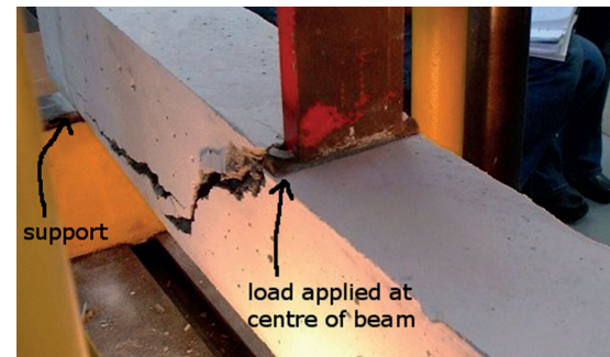
Figure 5.24 Shear cracks in a concrete beam – they start at the support.
