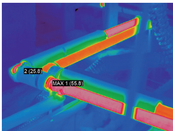
Figure 16.20 A thermal imaging camera detects thermal radiation. The hotter parts show up as orange and the cooler parts show up as blue. The image is formed by energy being radiated, rather than by light being reflected as in an ordinary camera.
